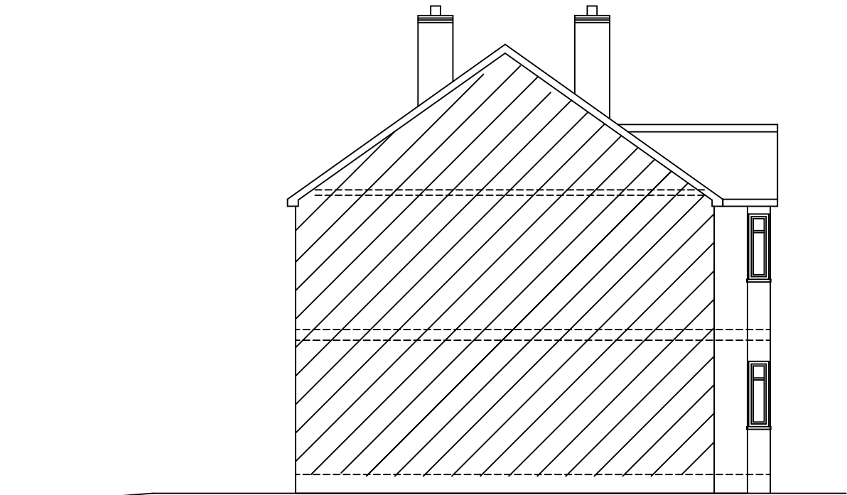
Existing Attached Elevation
