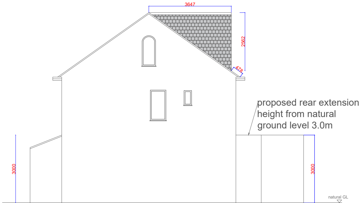
PROPOSED SIDE (SOUTH EAST) ELEVATION
