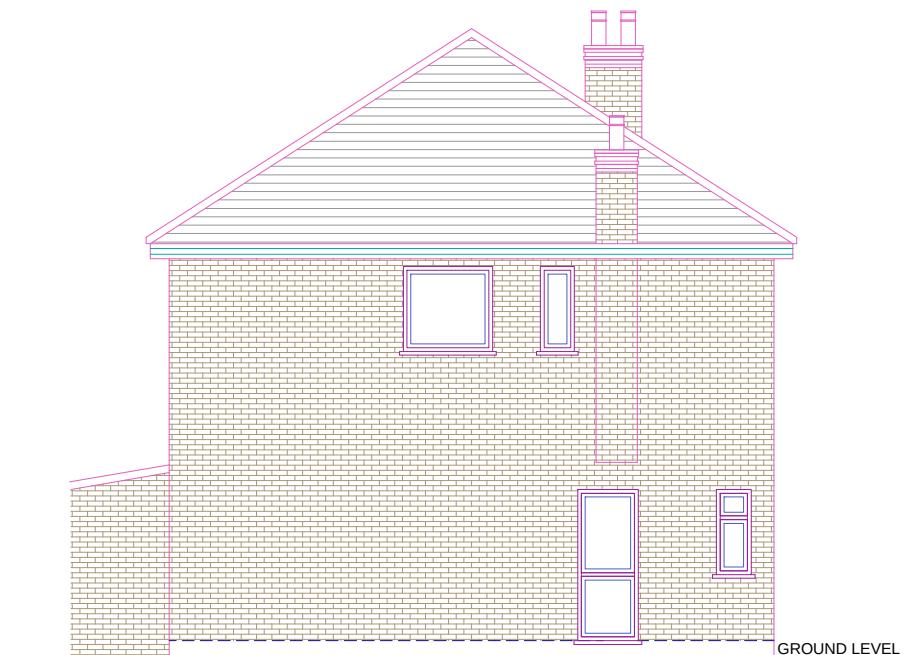
EXISTING ELEVATION SIDE A
