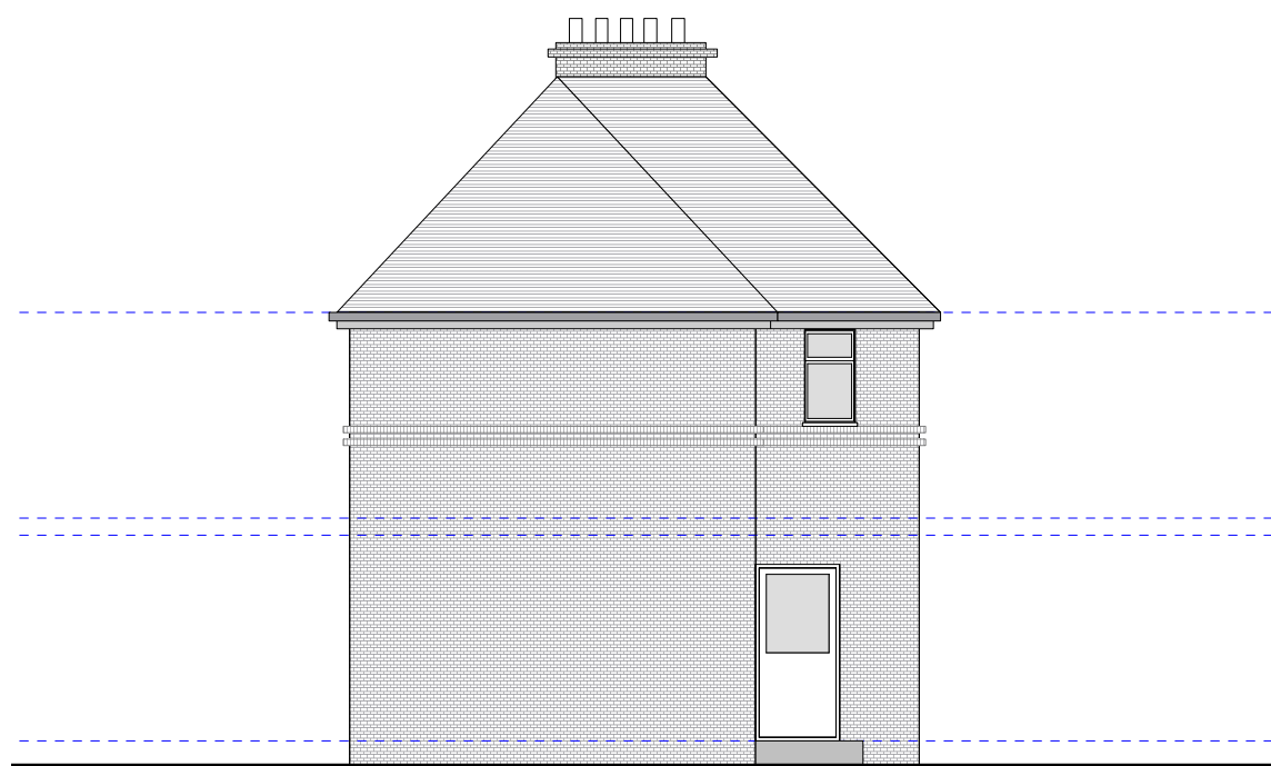
1 SIDE ELEVATION PLAN EX-20 Scale: 1/100
