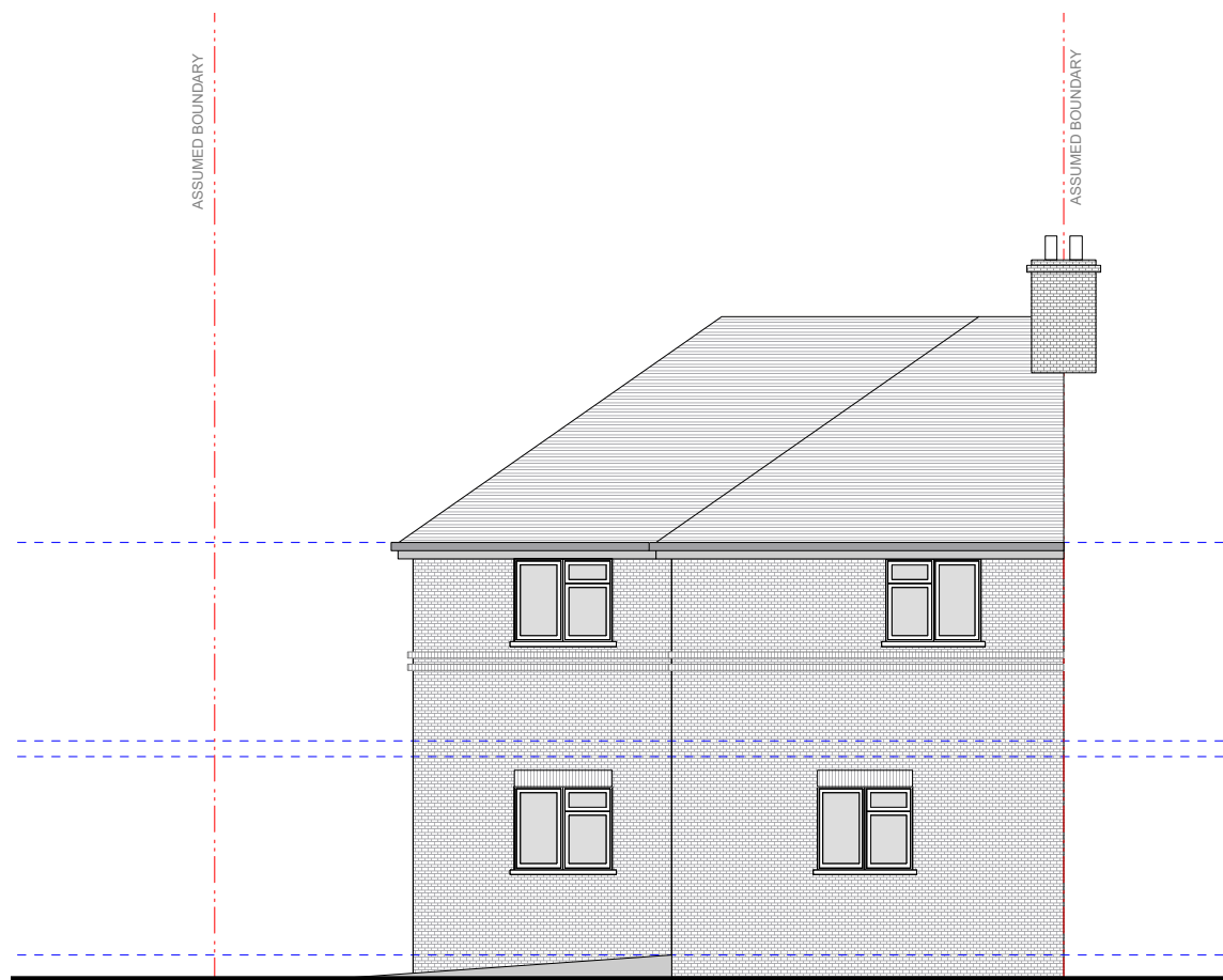
1 REAR ELEVATION PLAN EX-20 Scale: 1/100
