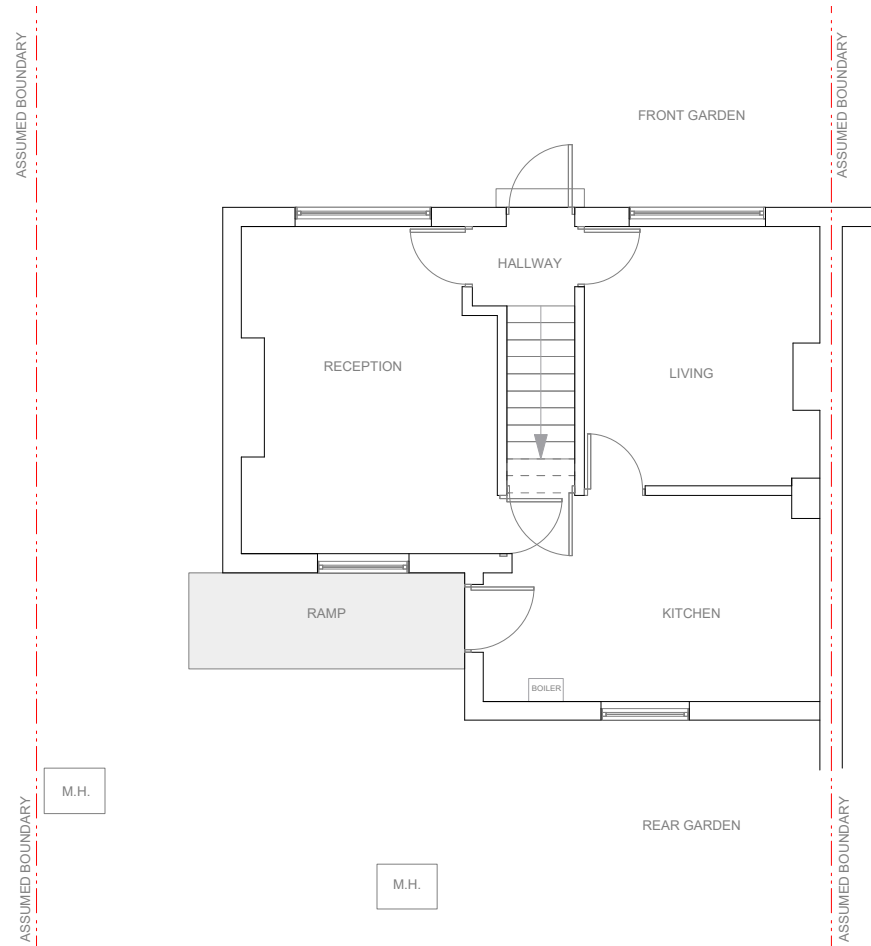
1 GROUND FLOOR PLAN EX-10 Scale: 1/100
