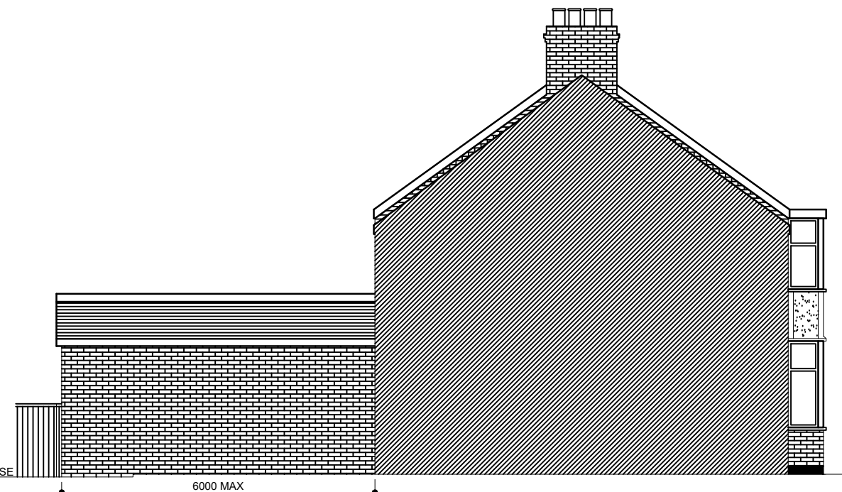
SIDE ELEVATION PROPOSED (AS VIEWED FROM NO:77)
