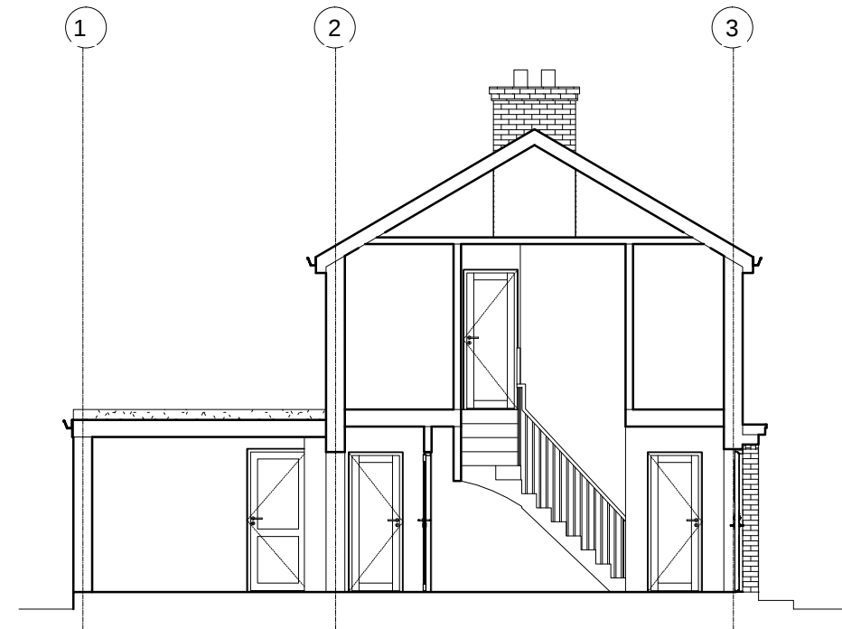
EXISTING SECTION
