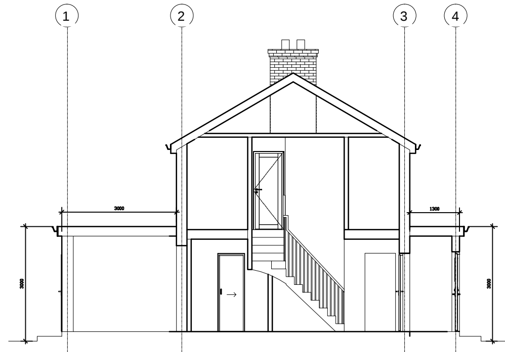
PROPOSED SECTION
