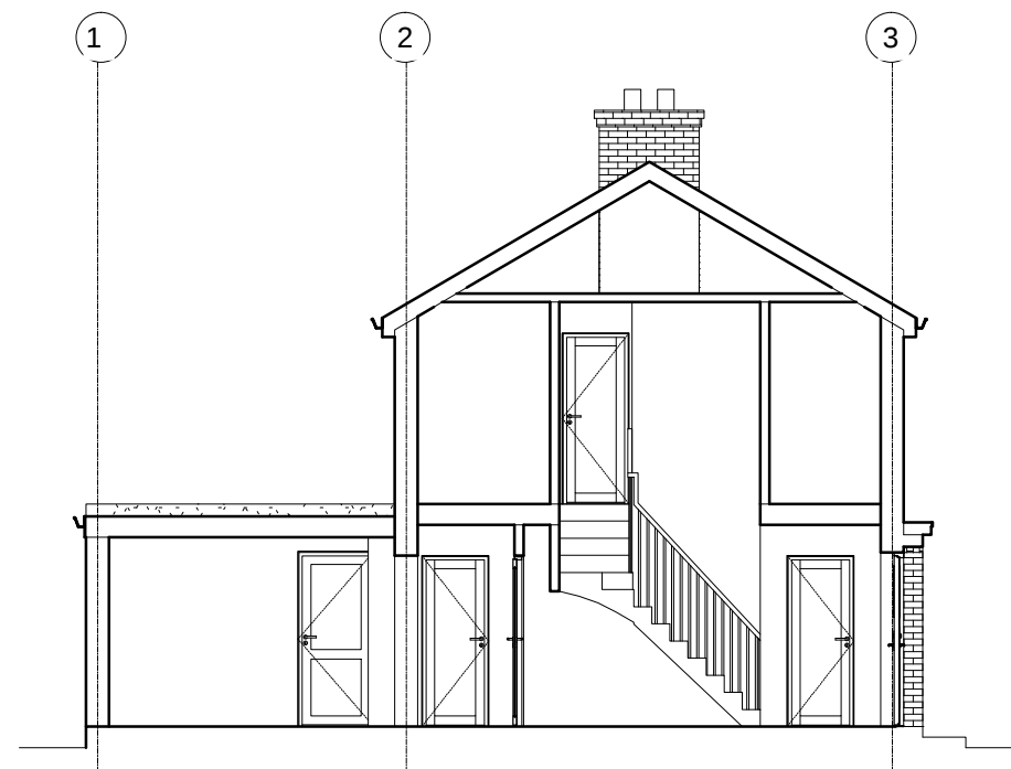
EXISTING SECTION
