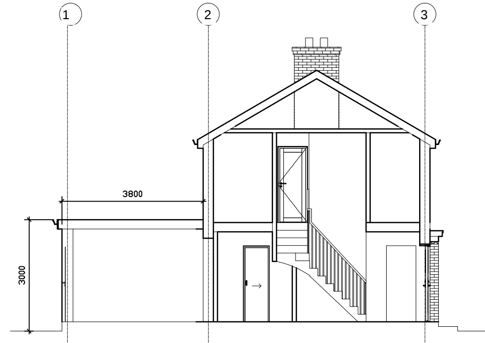
PROPOSED SECTION
