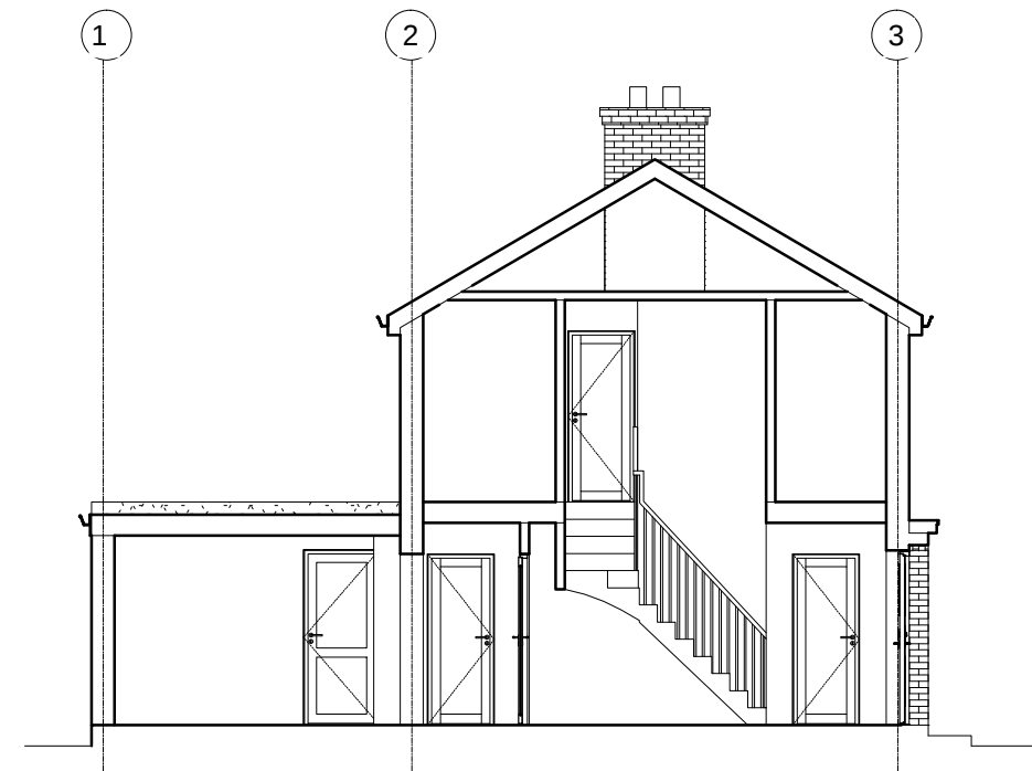
EXISTING SECTION
