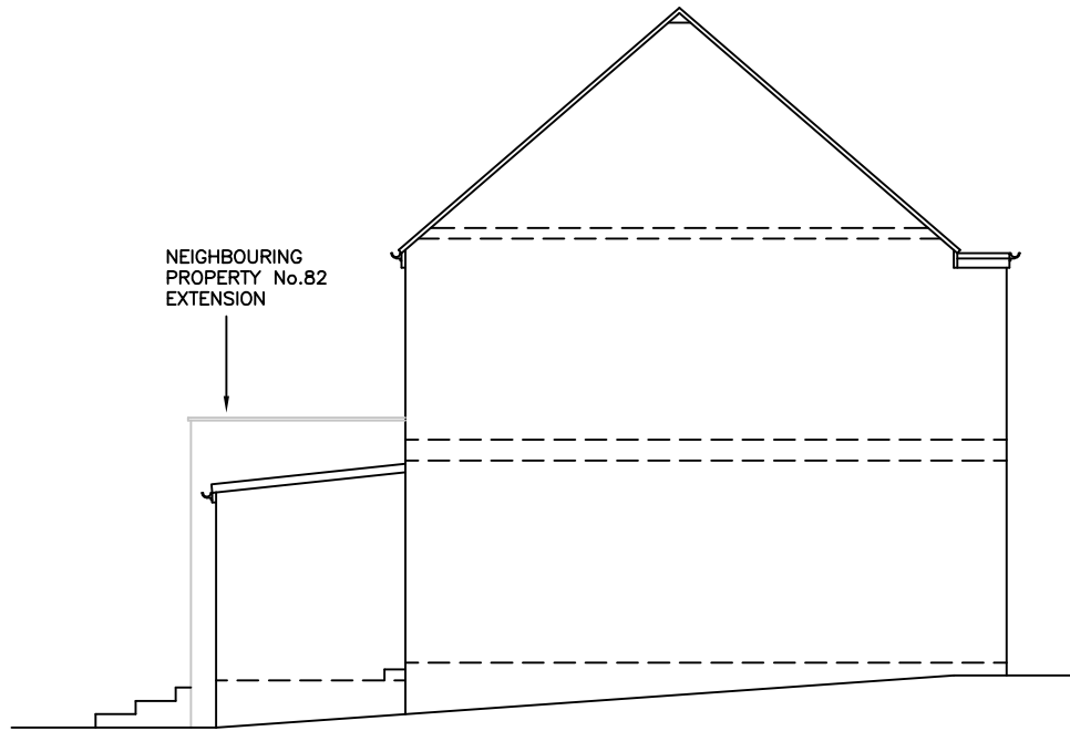
EXISTING OTHER SIDE ELEVATION
