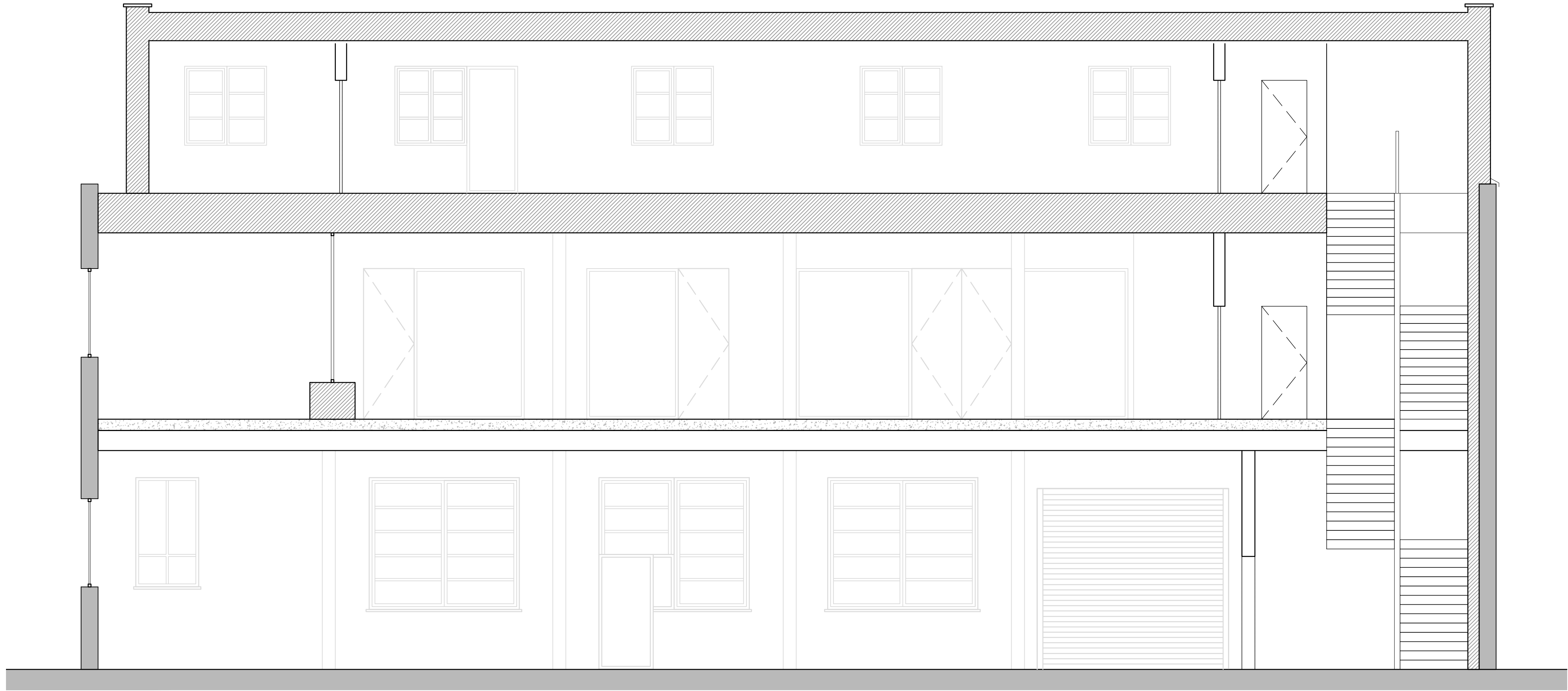
PROPOSED SECTION B-B' SCALE - 1:50 @ A1
