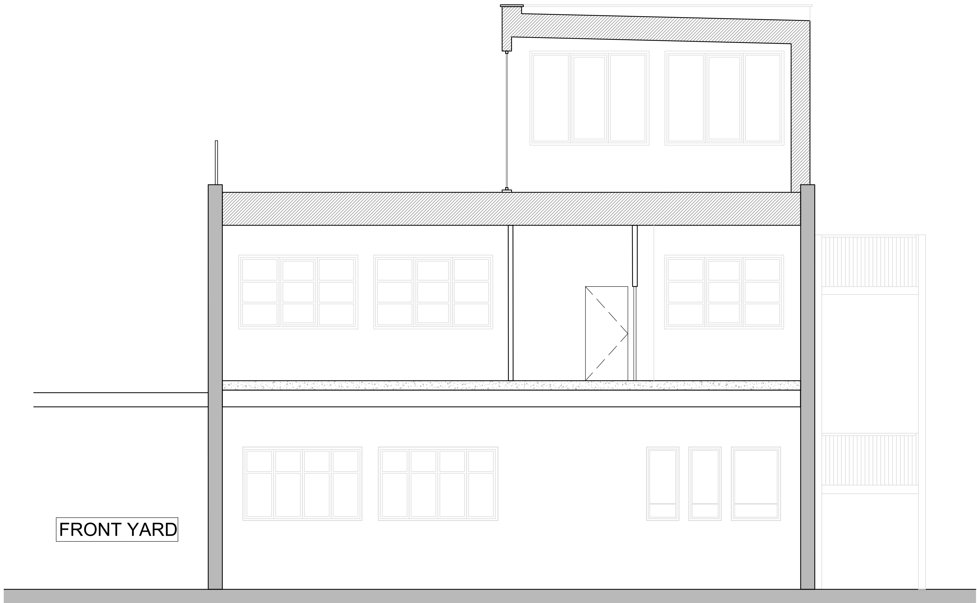
PROPOSED SECTION A-A' SCALE - 1:50 @ A1
