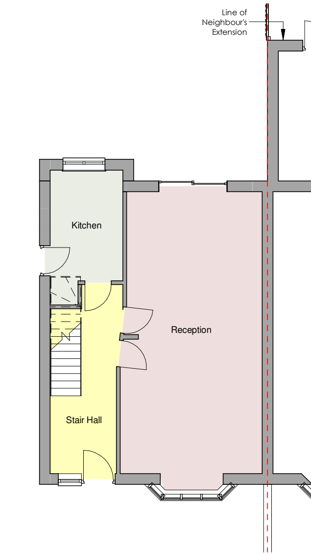
1 Ground Floor (Existing) 2312-A-200 1 : 100
