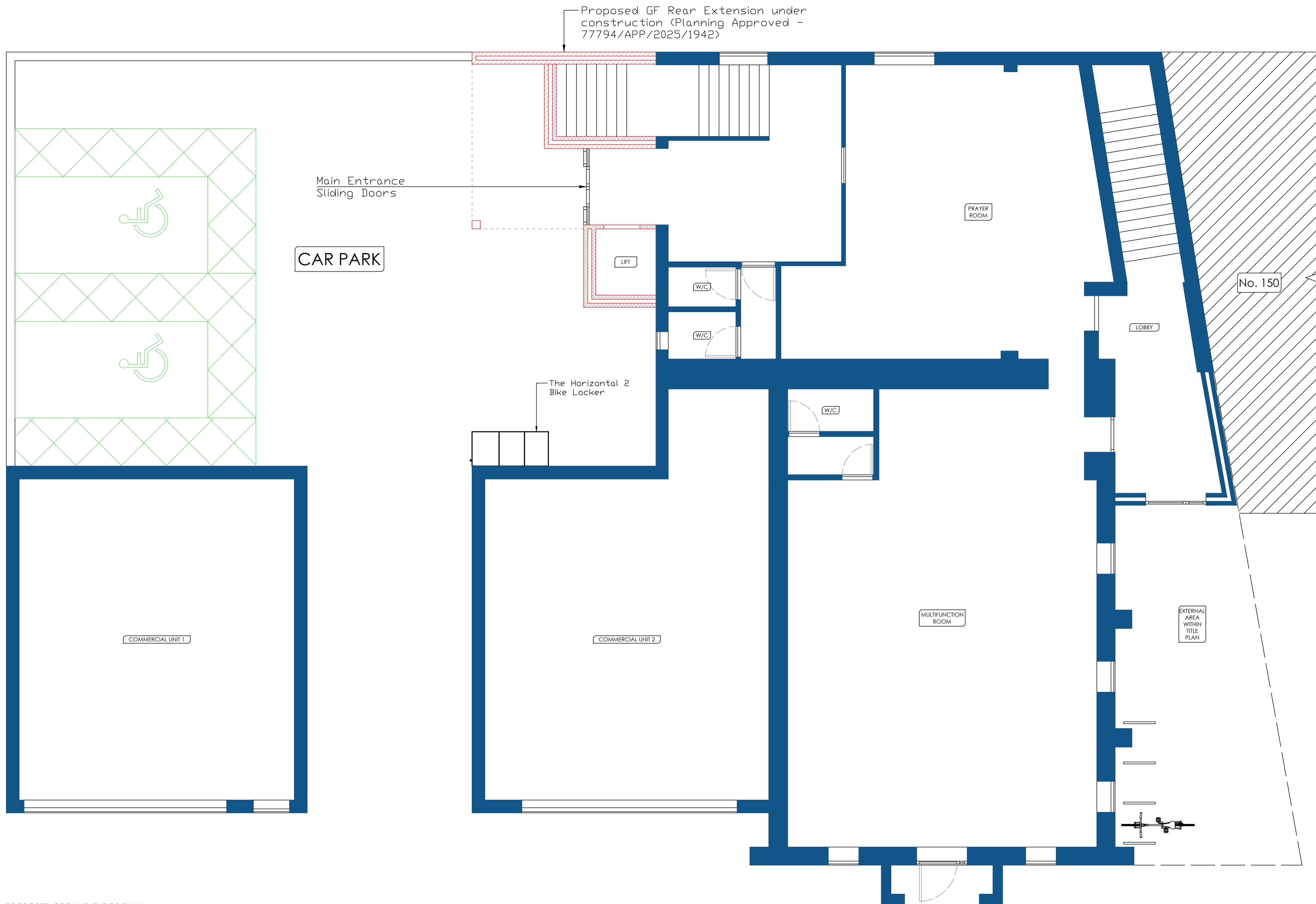
PROPOSED GROUND FLOOR PLAN SCALE 1:50
