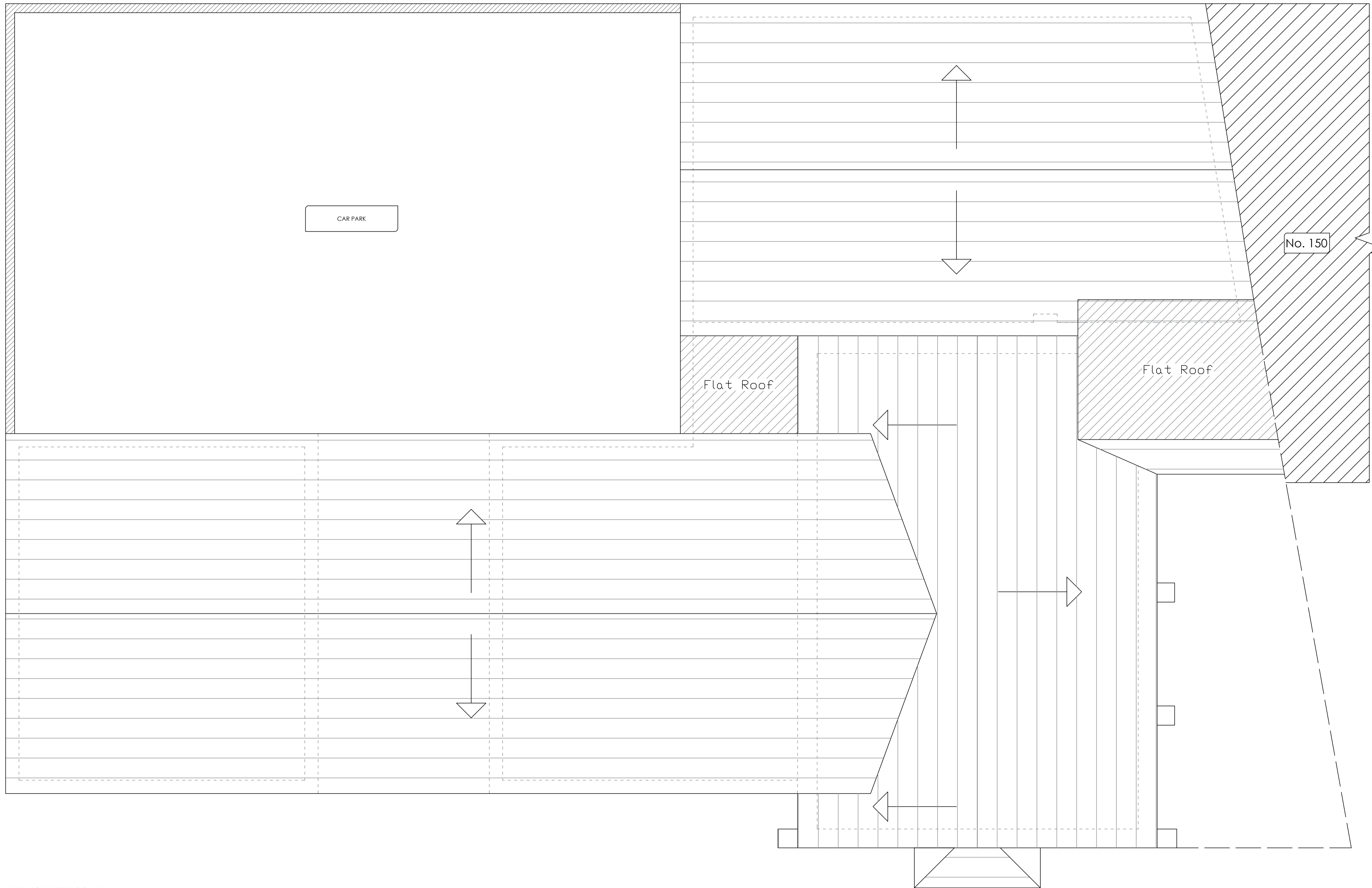
EXISTING FIRST FLOOR PLAN SCALE 1:50
