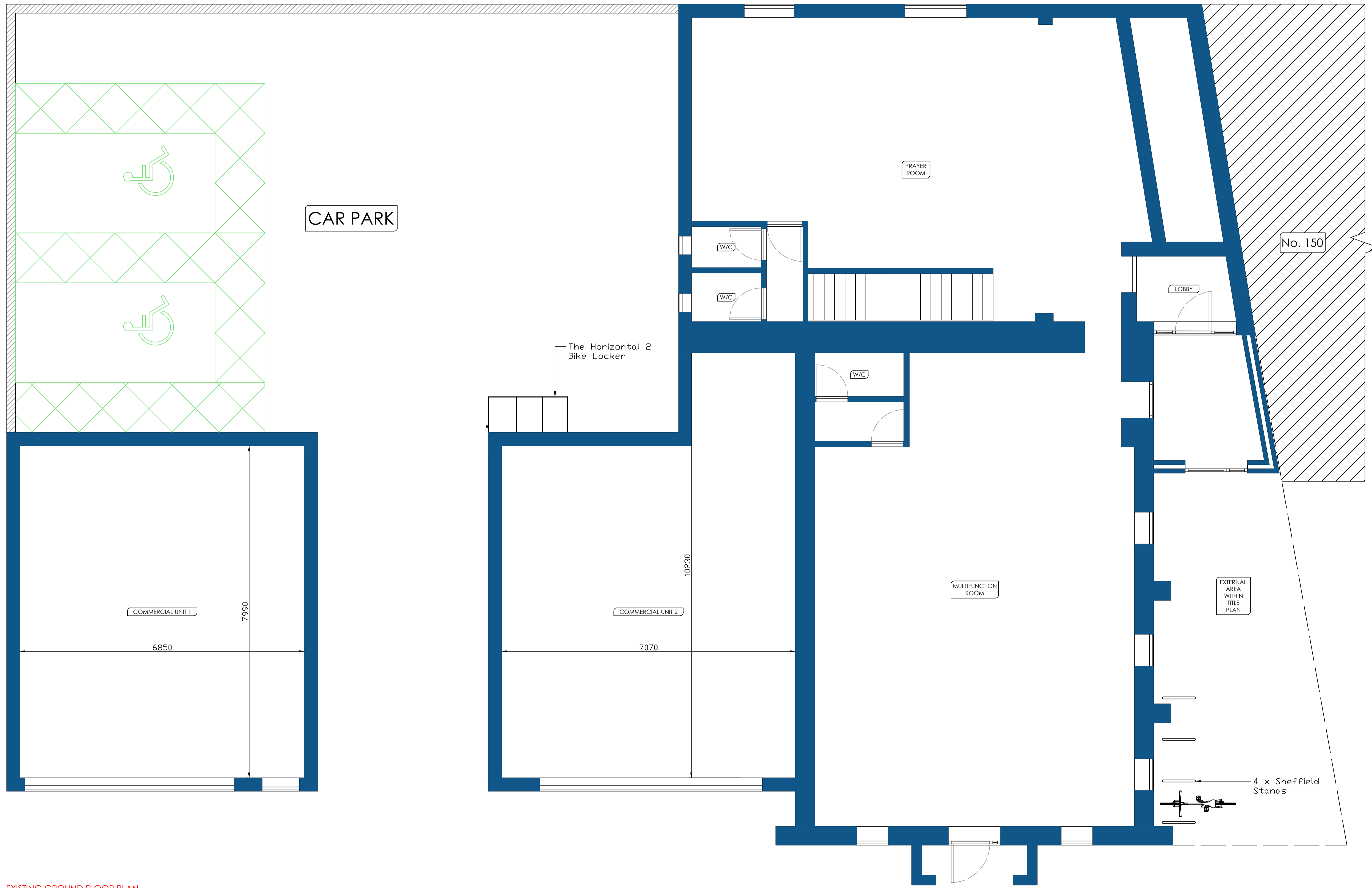
EXISTING GROUND FLOOR PLAN SCALE 1:50
