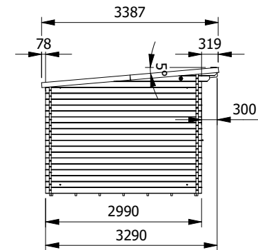
Elevation D Scale 1:100
