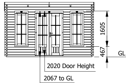
Elevation A Scale 1:100
