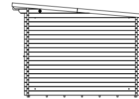
Elevation D Scale 1:100
