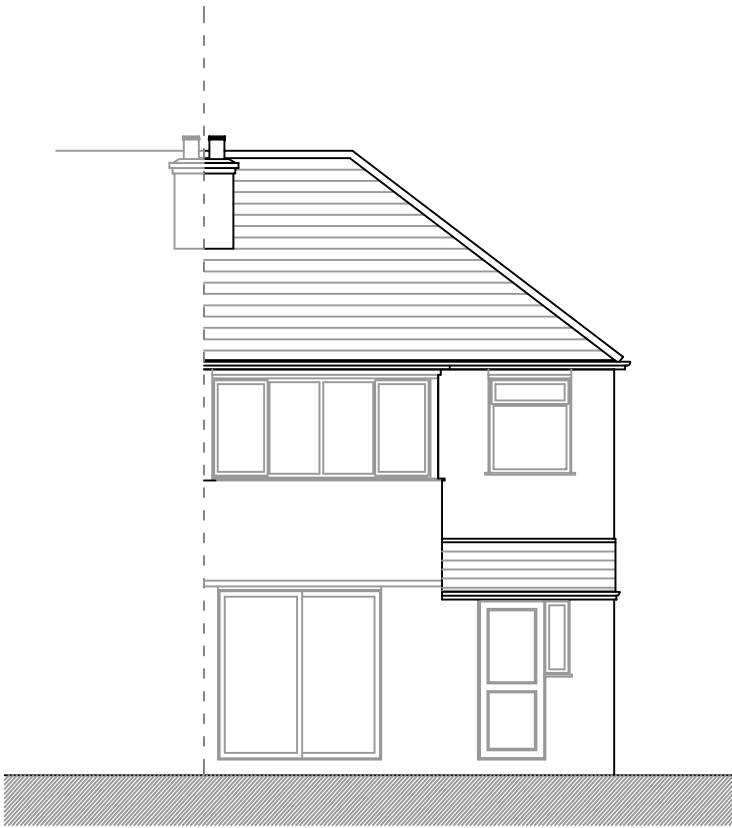
EXISTING BACK ELEVATION
