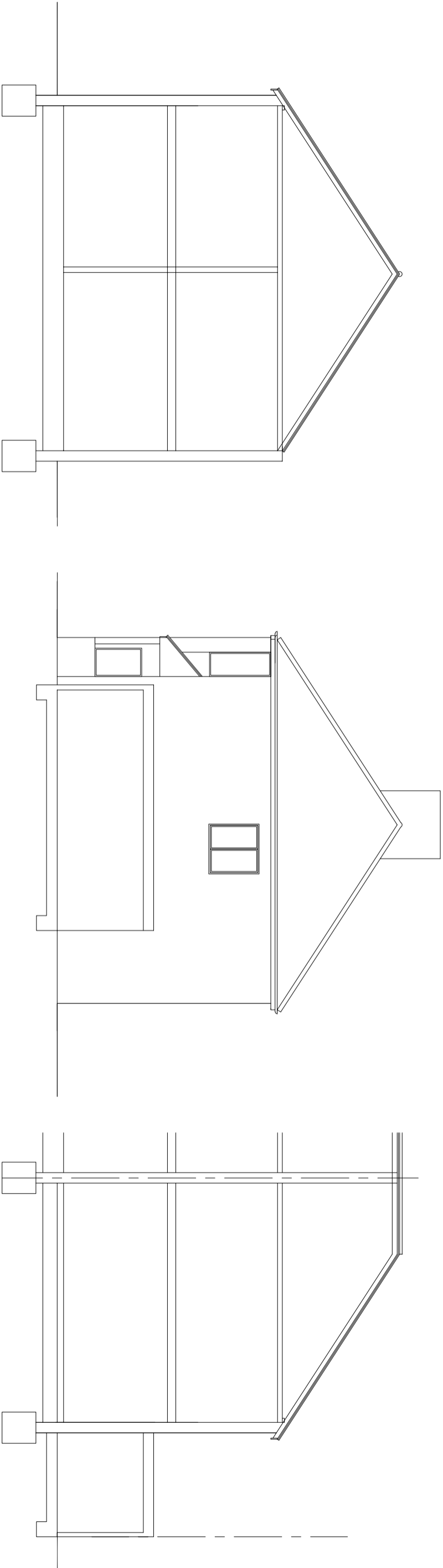
SECTION A
