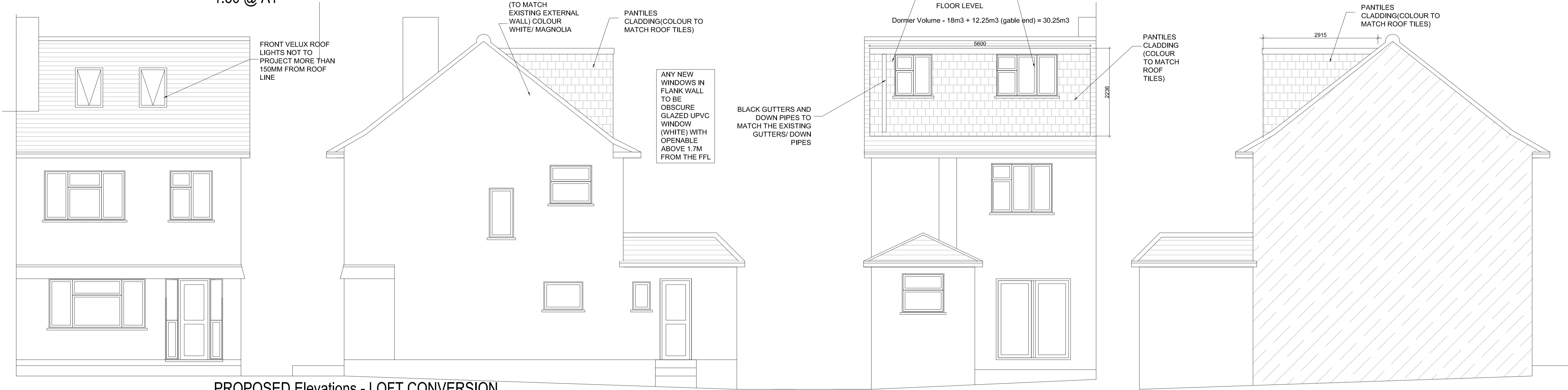
PROPOSED Elevations - LOFT CONVERSION 1:50 @ A1
