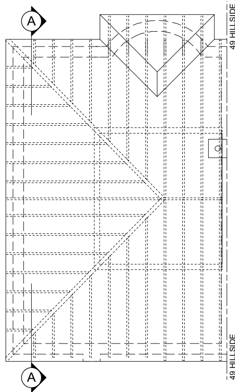
EXISTING LOFT PLAN
