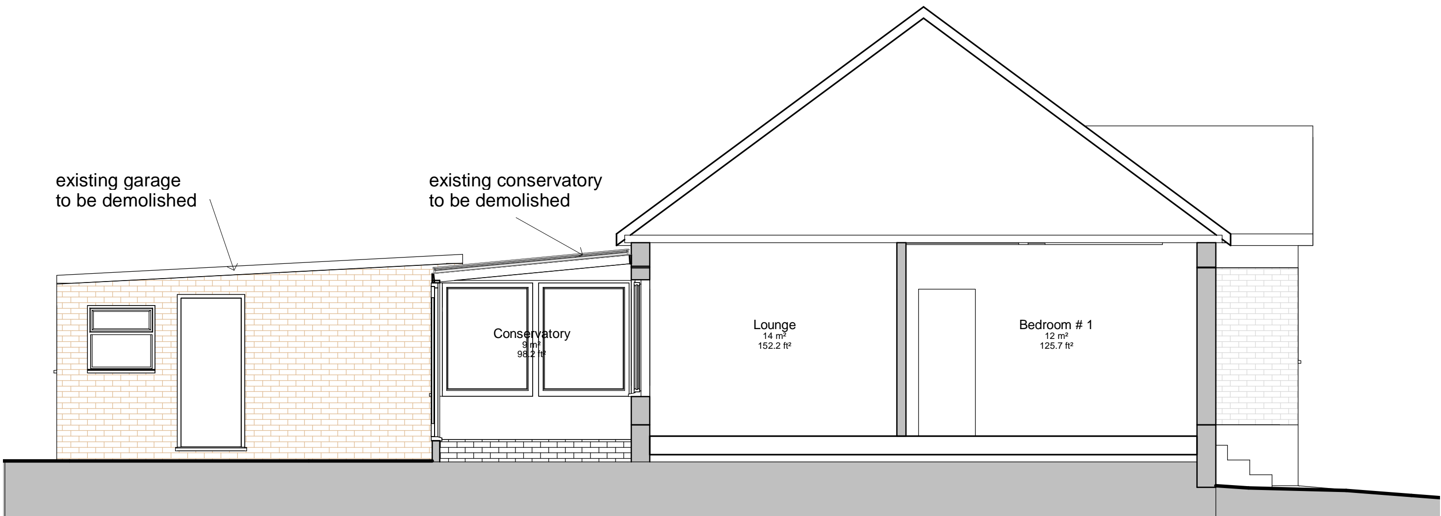
Existing Section
