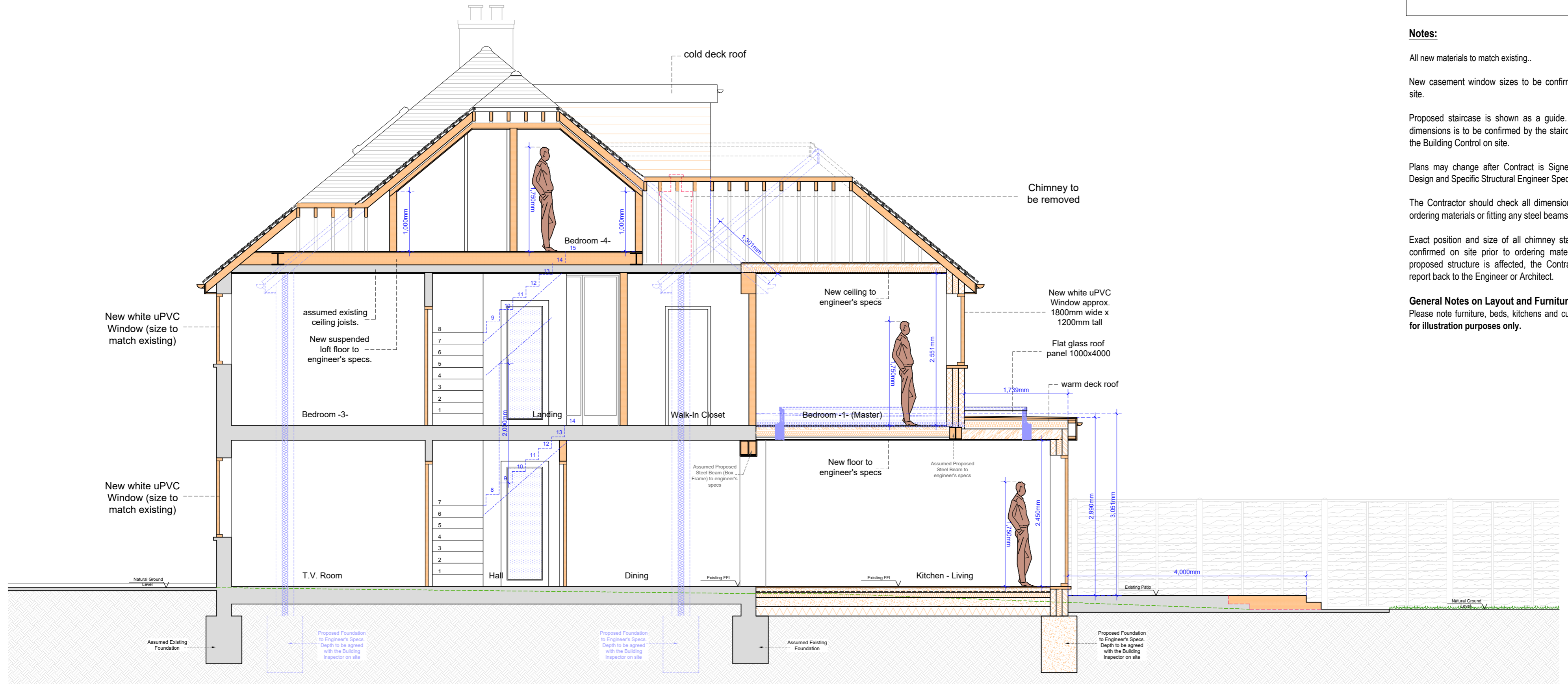
PROPOSED SECTION A-A
