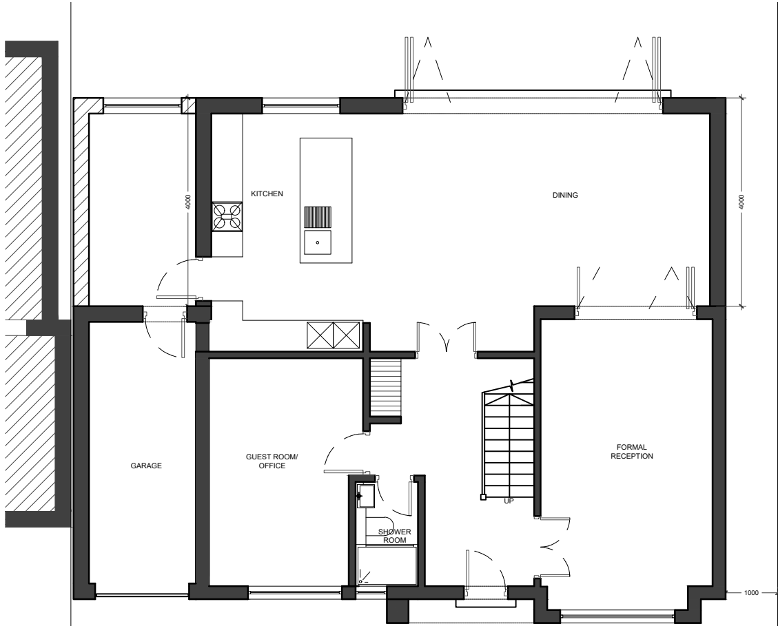
01 - GROUND FLOOR PLAN
