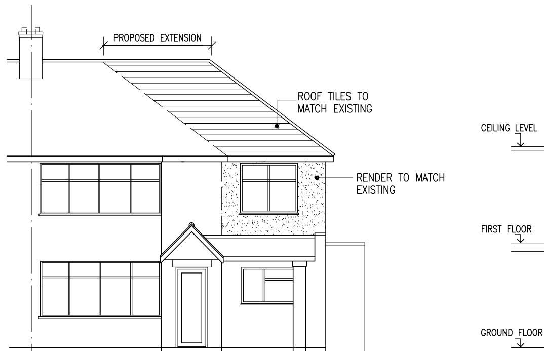
FRONT ELEVATION
