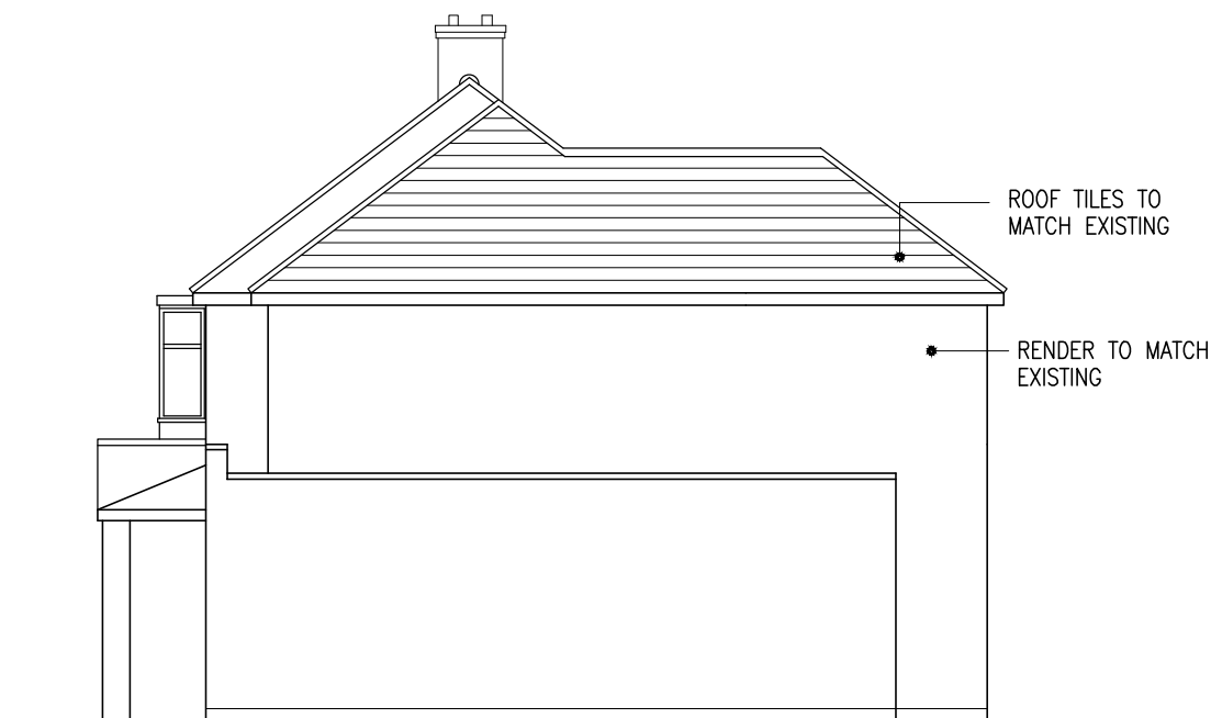
SIDE ELEVATION
