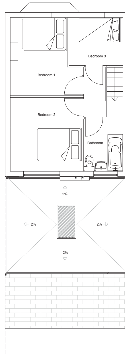
PROPOSED ROOF 1:100
