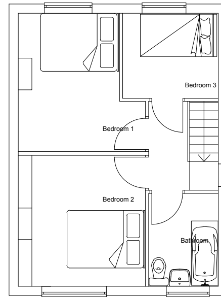
EXISTING FF 1:100
