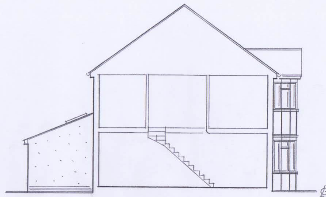
SOUTH - WEST SIDE ELEVATION
