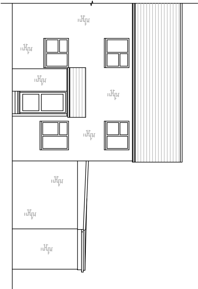
NORTH ELEVATION
