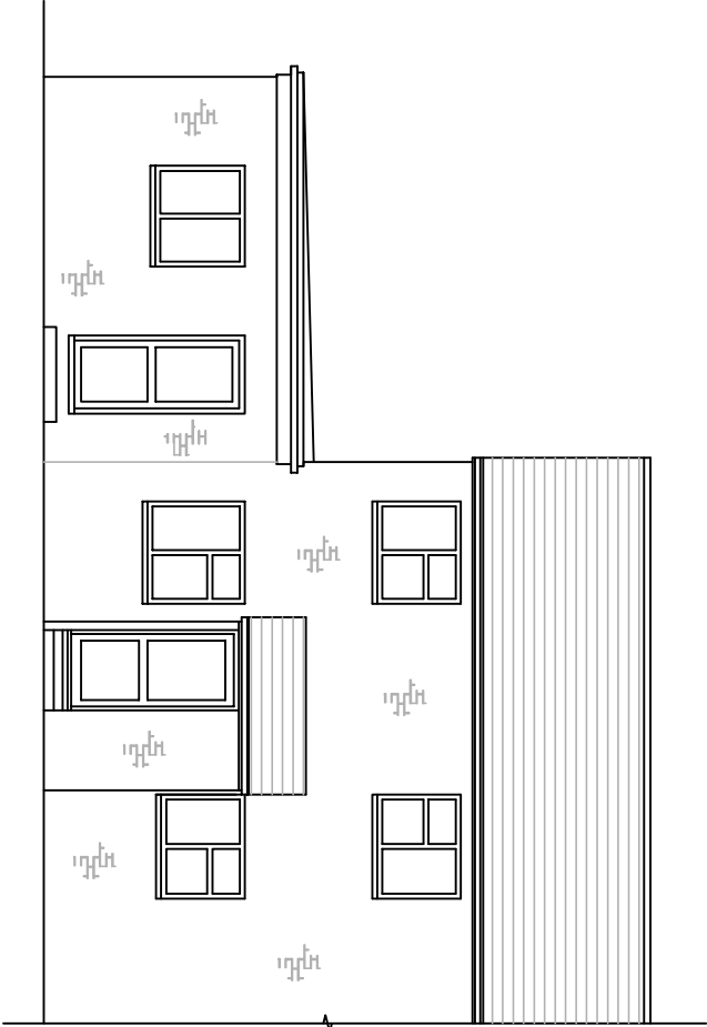
SOUTH ELEVATION
