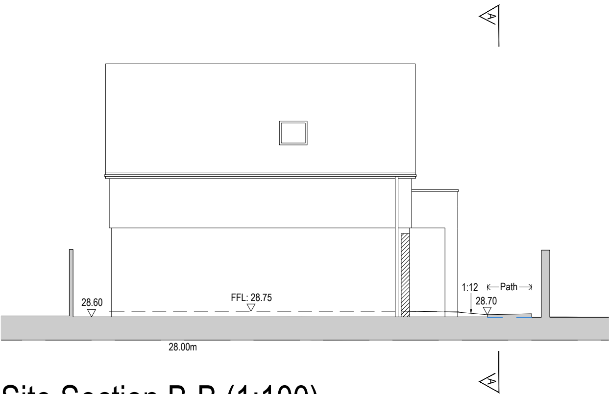
Site Section B-B (1:100)
