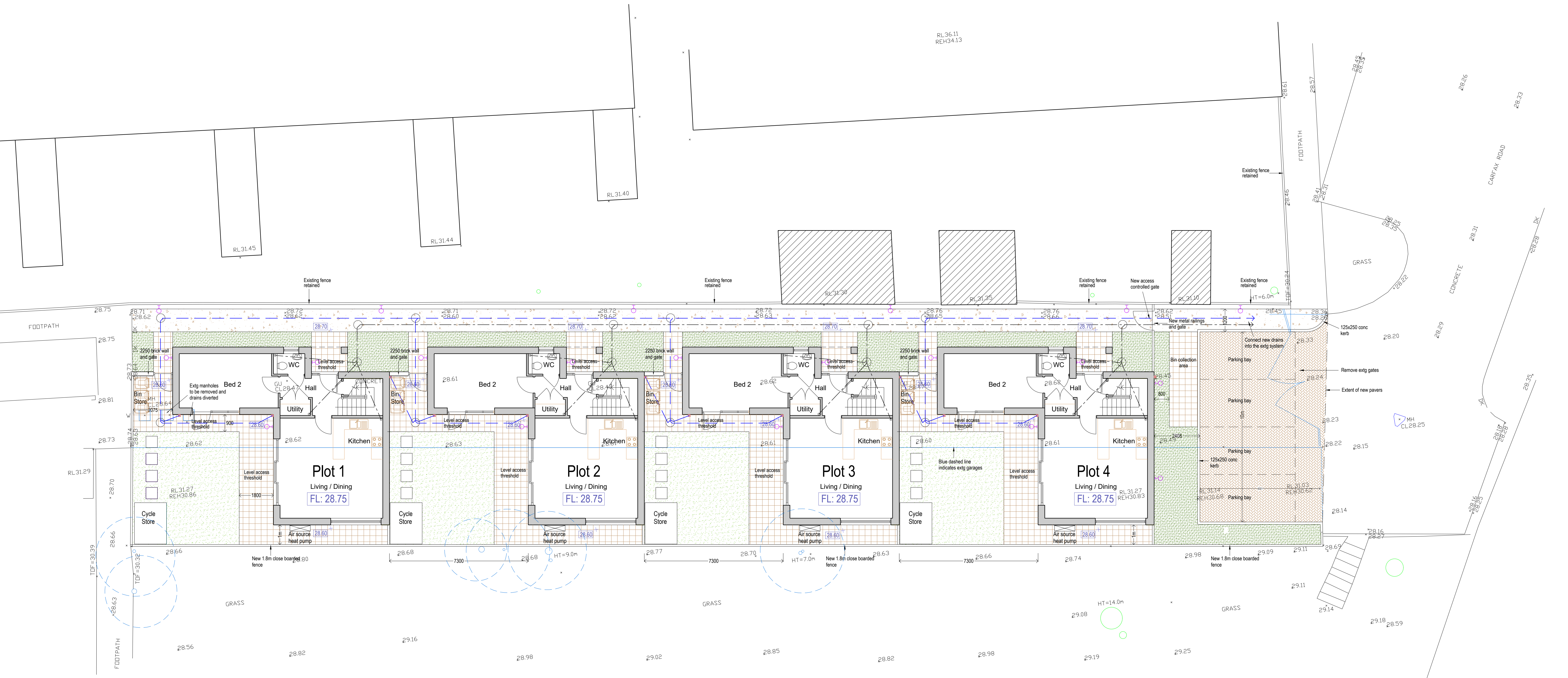
Site plan (1:100)
