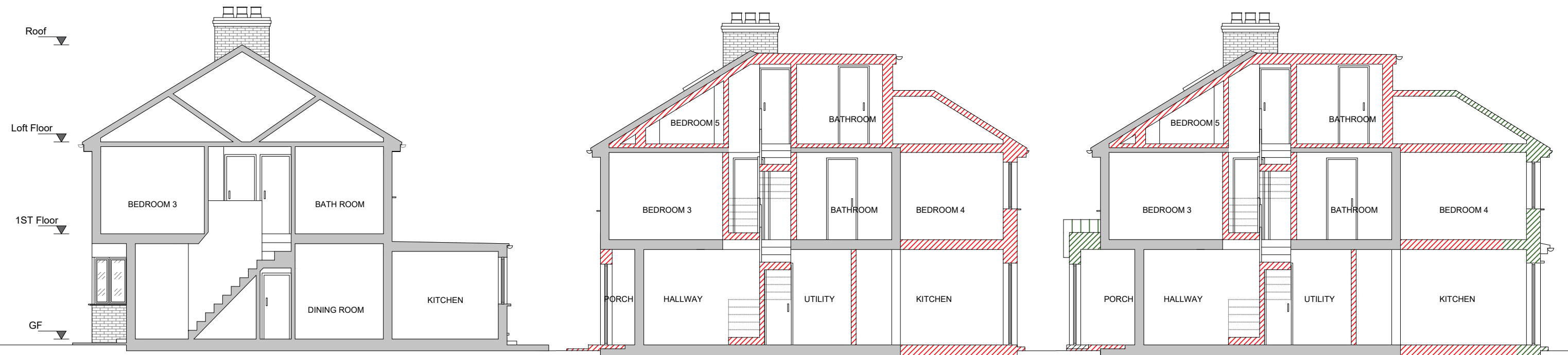
APPROVED SECTION A - A (Ref:77427/APP/2023/2946) scale 1:100
