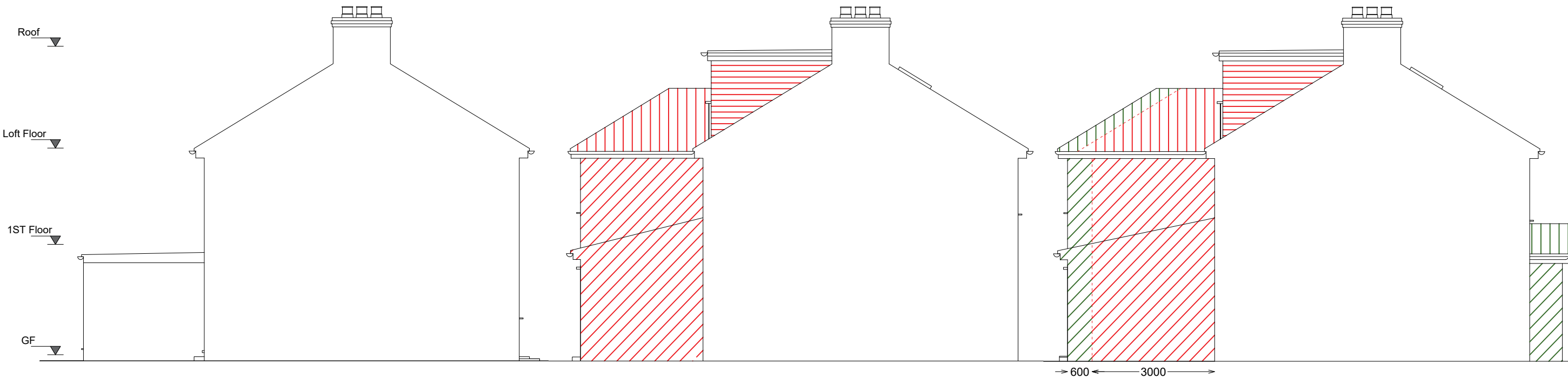
APPROVED REAR ELEVATION - A (Ref:77427/APP/2023/2946) scale 1:100
