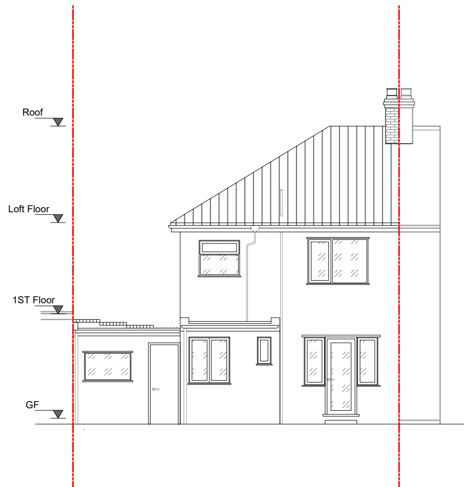
EXISTING REAR ELEVATION scale 1:100
