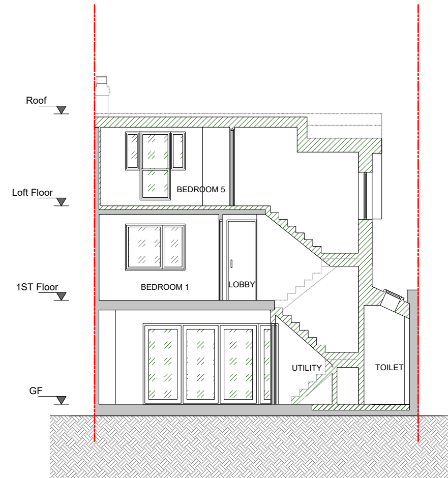
PROPOSED SECTION B - B scale 1:100
