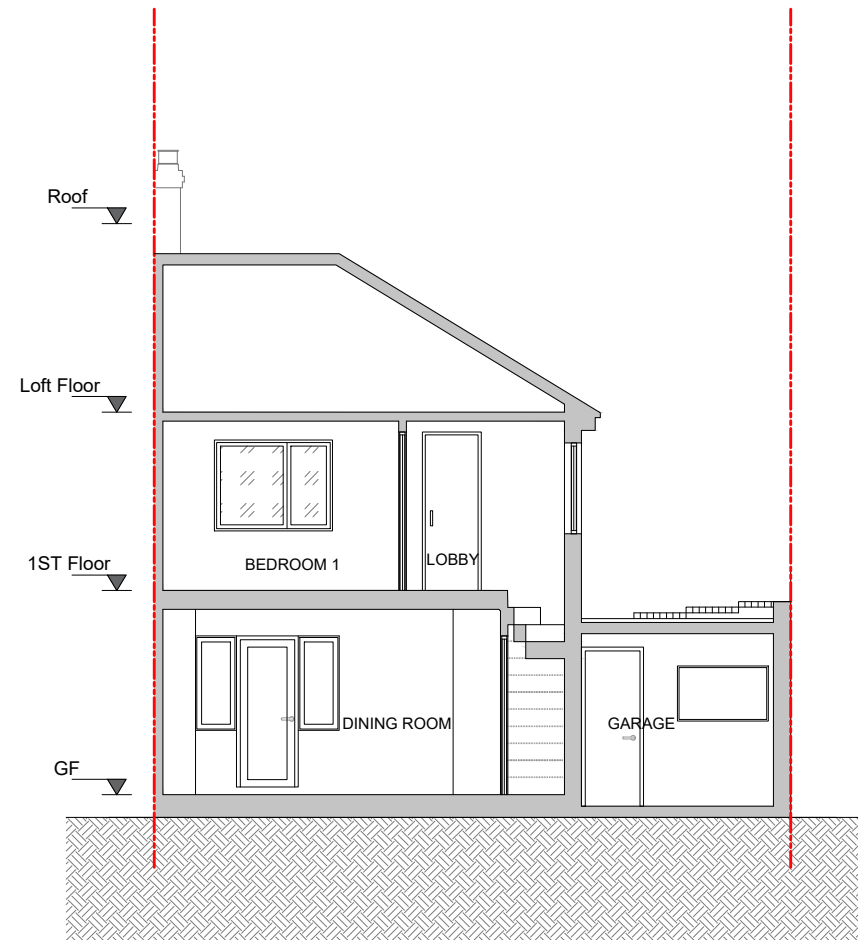
EXISTING SECTION B - B scale 1:100
