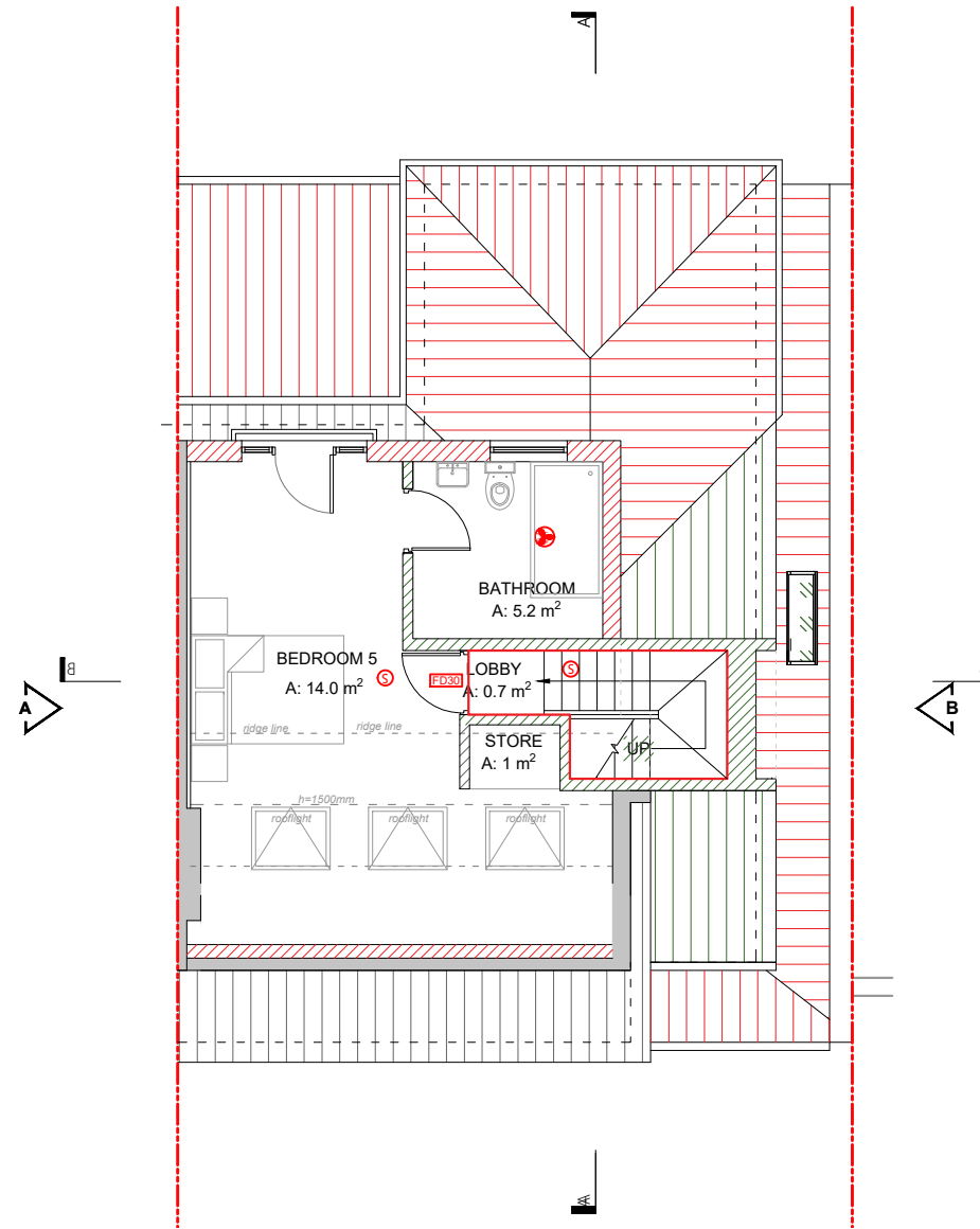
PROPOSED LOFT FLOOR PLAN Combine with both approved scale 1:100
