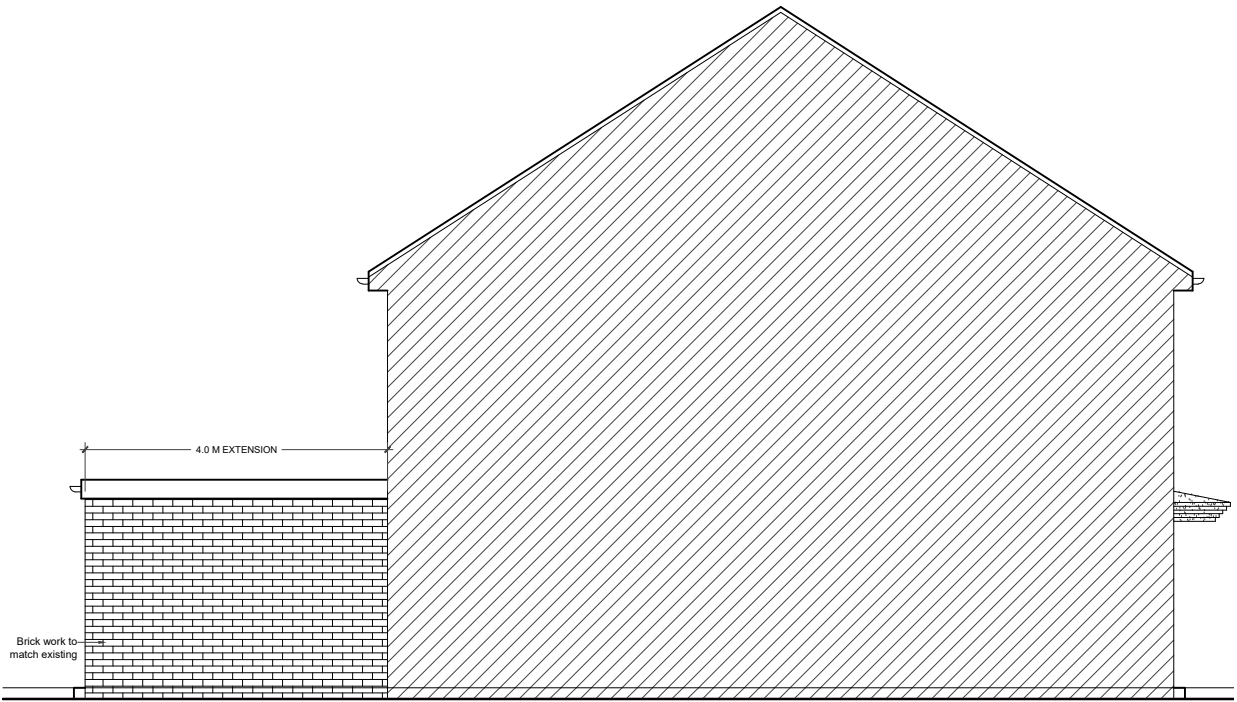
04 - SIDE ELEVATION
