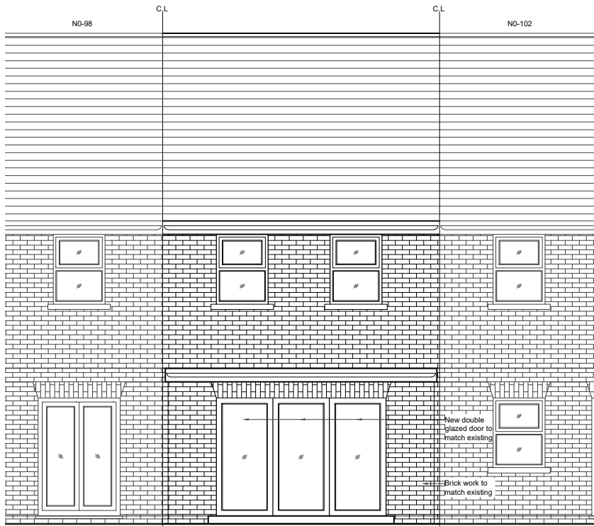
03 - REAR ELEVATION
