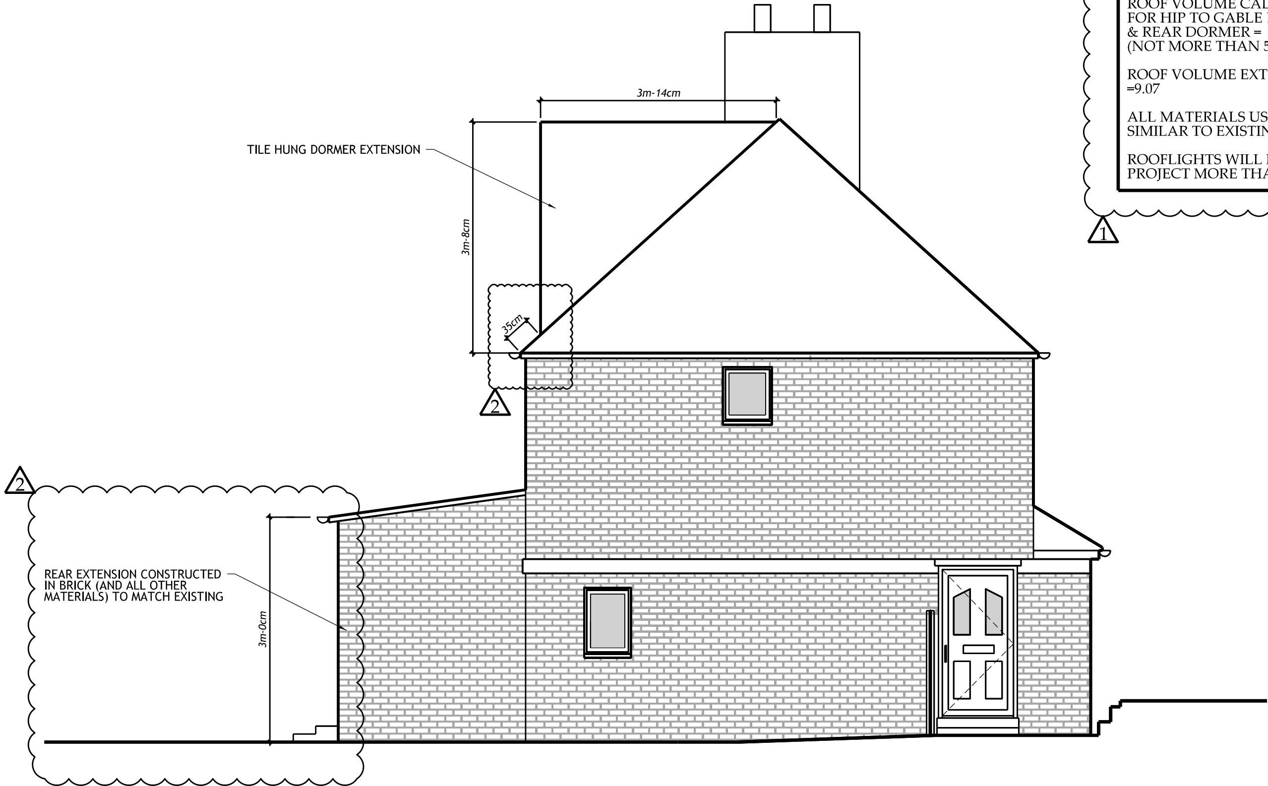
1 A302 PROPOSED SIDE ELEVATION SCALE: 1:50
