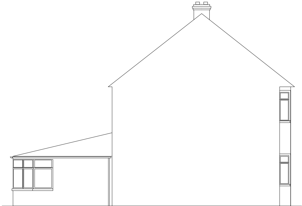
901 EXISTING SIDE ELEVATION -
