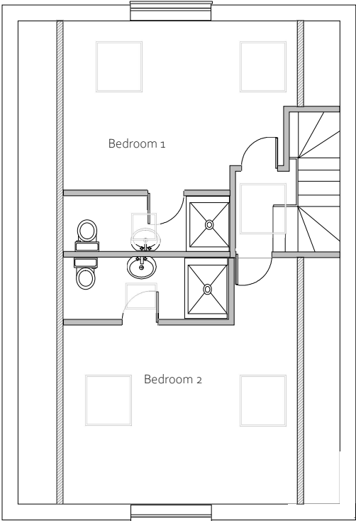
rear side of property Proposed Loft Floor Plan
