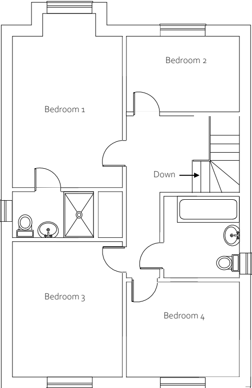
Rear Side of property Existing First Floor Plan Front Side of property
