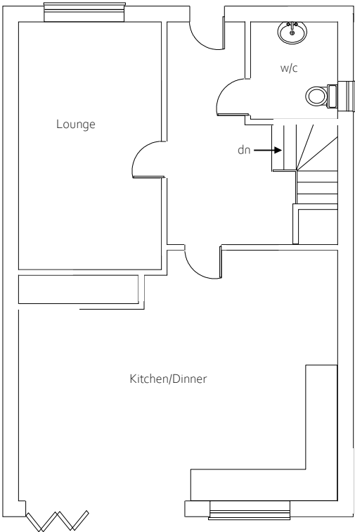
Rear Side of property Existing Ground Floor Plan
