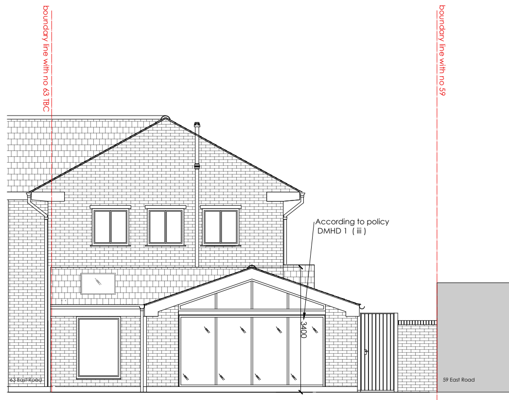
ELEVATION BB - proposed
