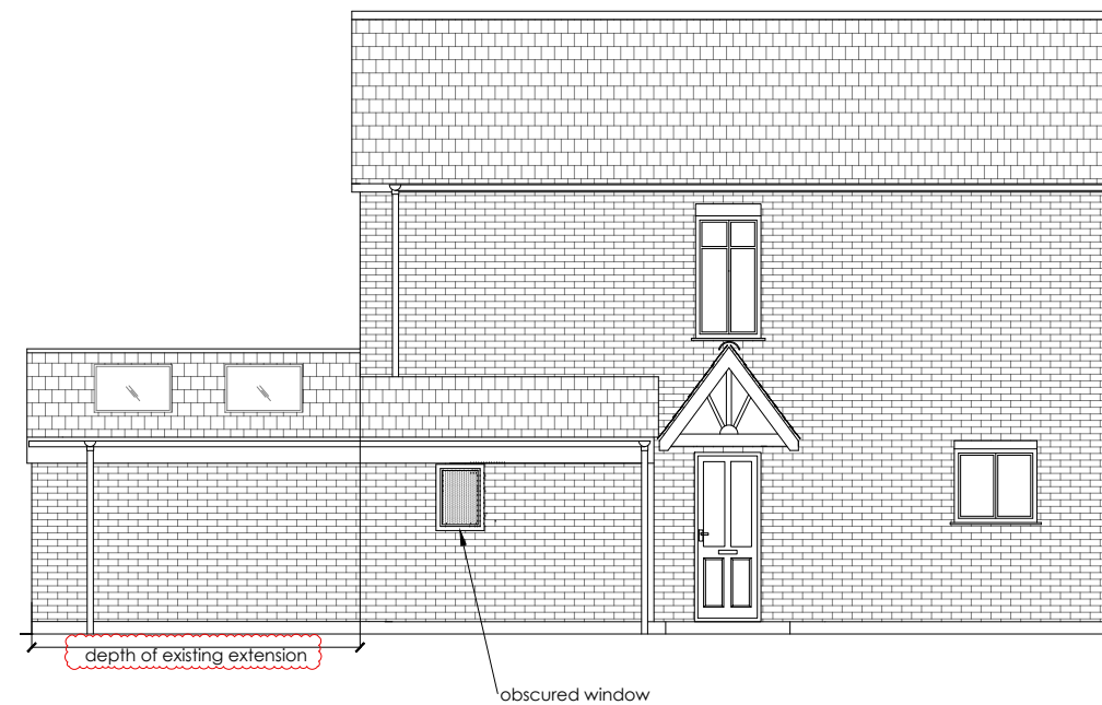
ELEVATION DD - proposed
