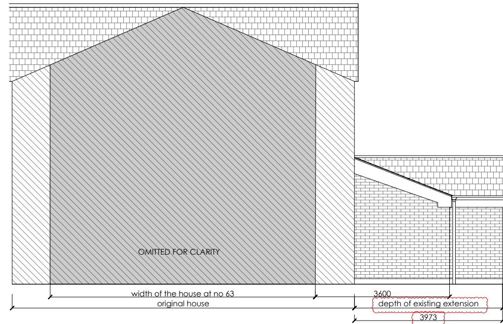
ELEVATION CC - proposed
