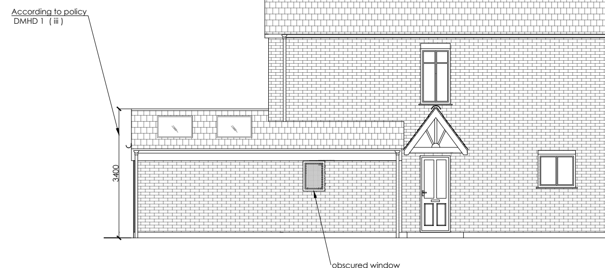
ELEVATION DD - proposed
