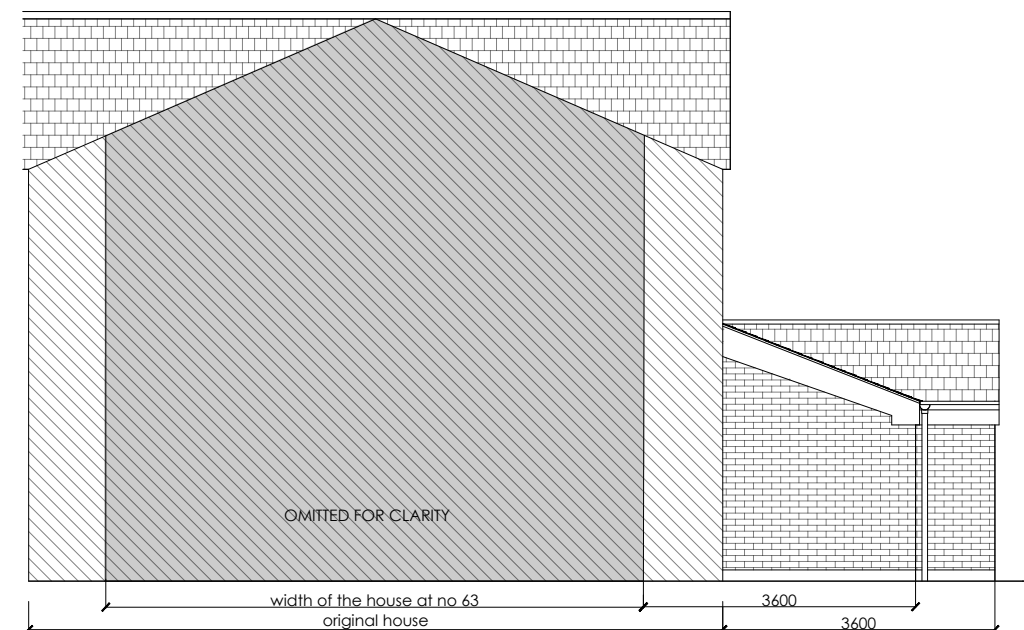
ELEVATION CC - proposed
