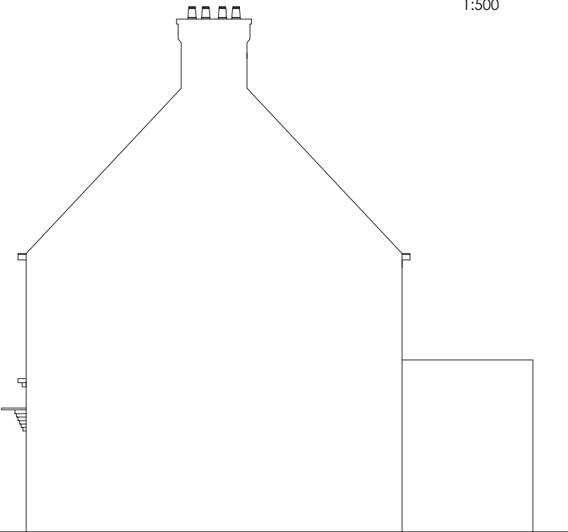
EXISTING SIDE (PARTY WALL) ELEVATION
