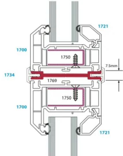
1769 - Structural Coupler & 1734 - Cover Trim
