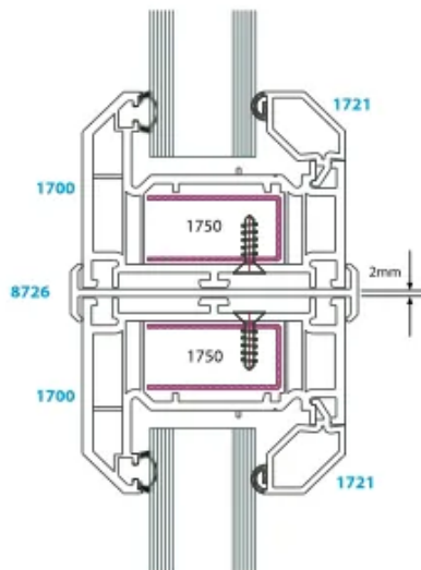
8726 - 'H' Coupler Connecting Profile
