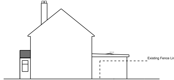
Proposed Right Hand Elevation
