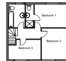
First Floor Proposed
