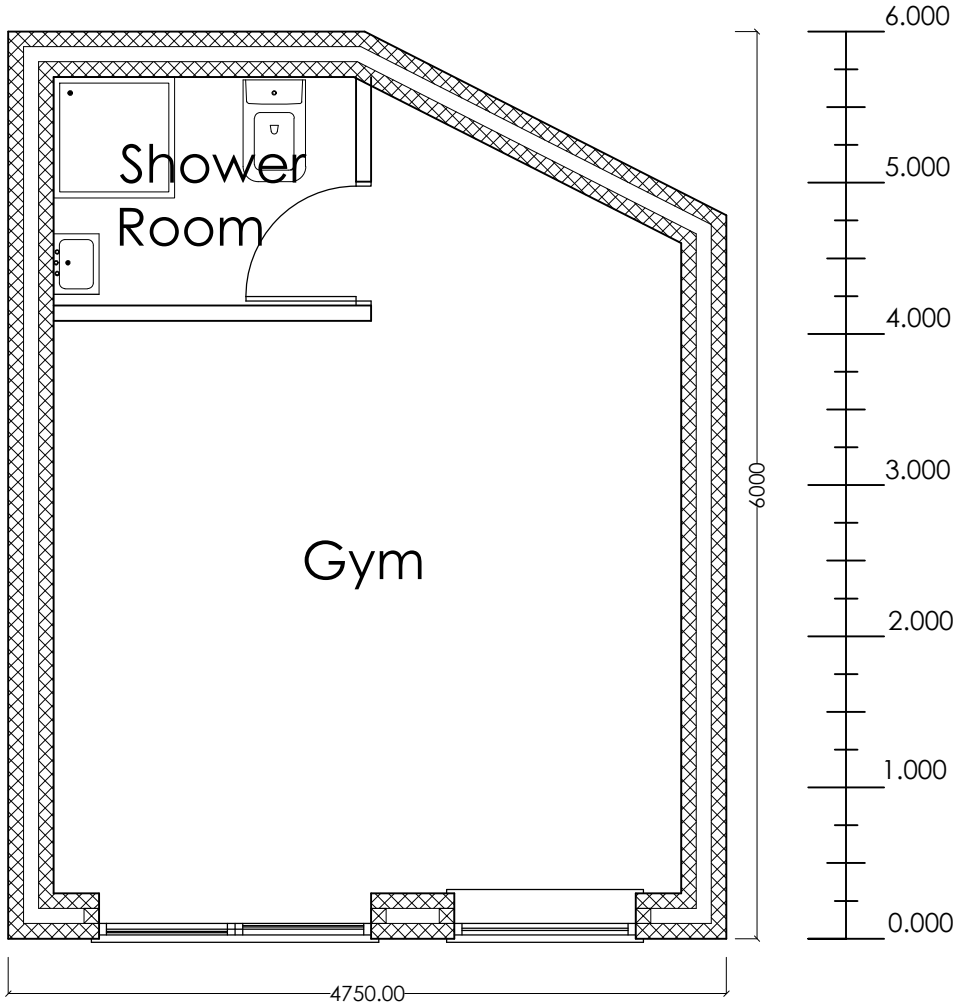
Floor Plan
