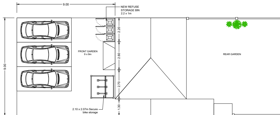
PROPOSED SITE PLAN 1:200
