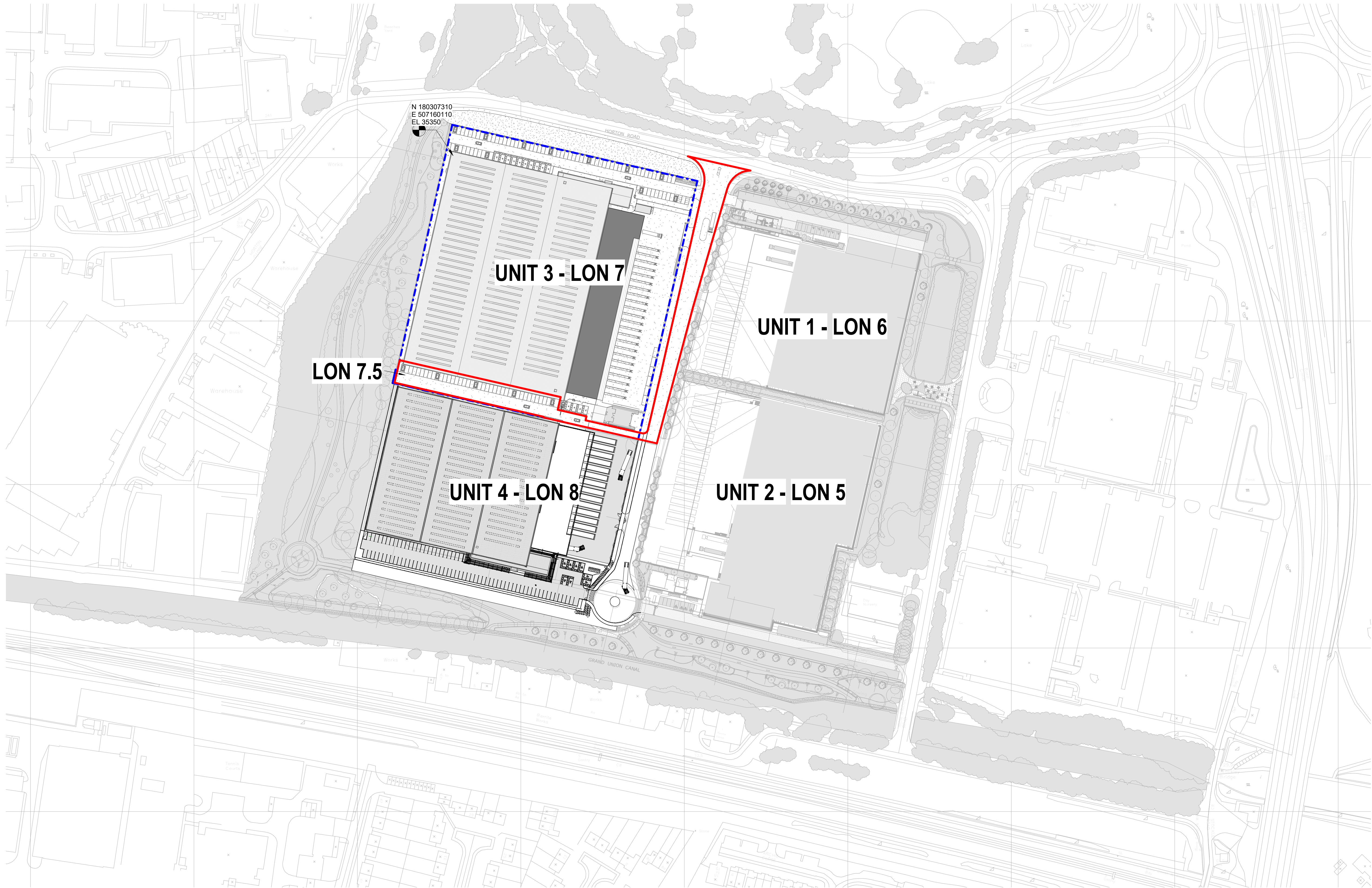
① LOCATION PLAN - EXISTING 1 : 1250
